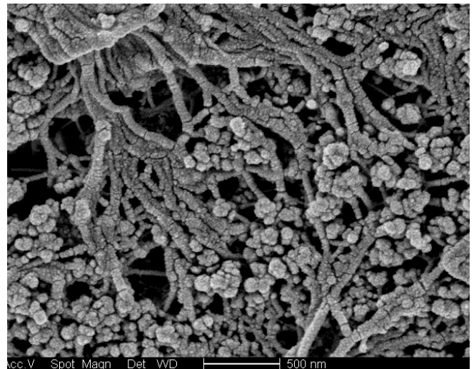
SEMs - ENTEK LR Separator
